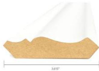
MOLDING CROWN M AVAILABLE IN 3.615" SIZE
